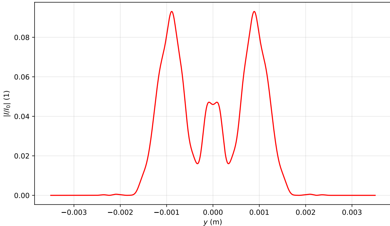
Intensity profile I(x=0, y, z=2.627)/I_0 , P_{in}=7.5P_{cr} , artificial time
